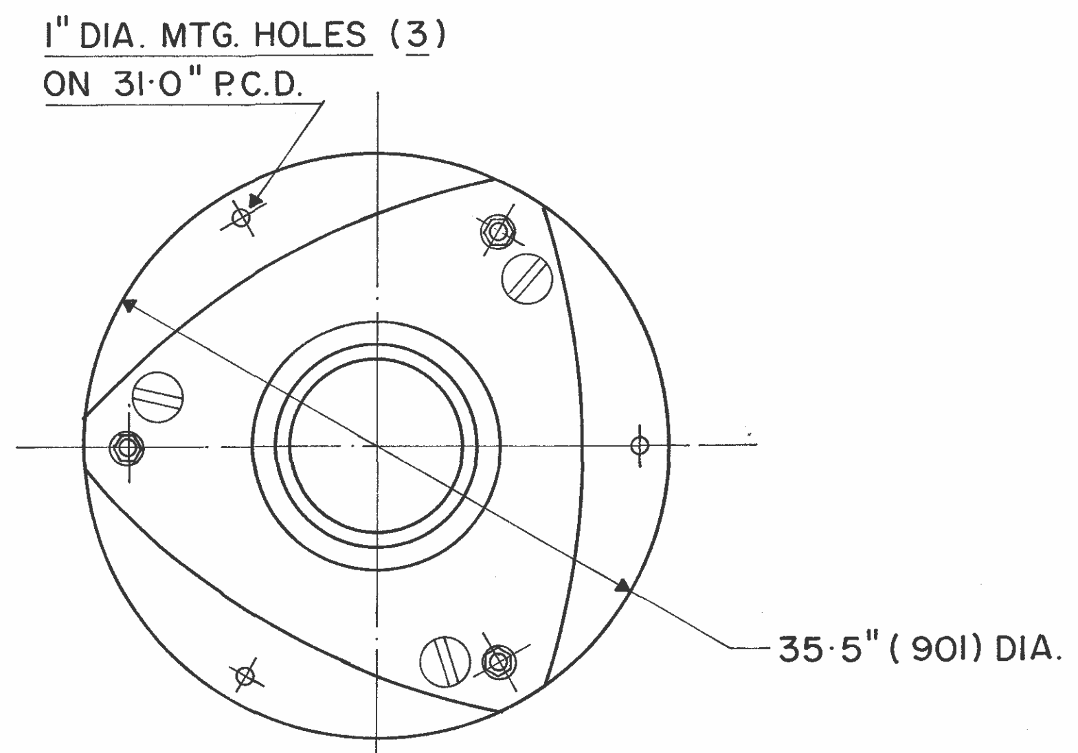
TOP VIEW OF COMMUNUTOR
