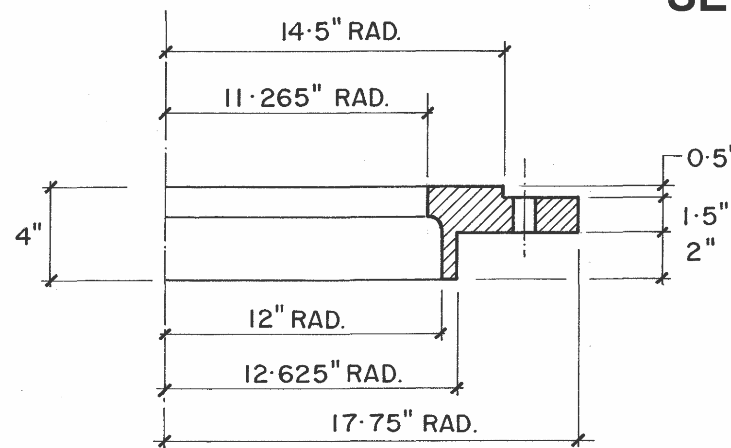
BASE RING DETAIL
